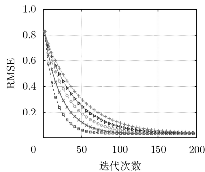
(b) RMSE
