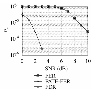
图5 N=256 , NSI-IPR-OFDM
