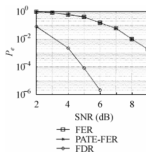
图4 N=64 , NSI-IPR-OFDM
