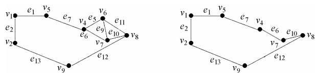
(a) G_0 (b) G_1
